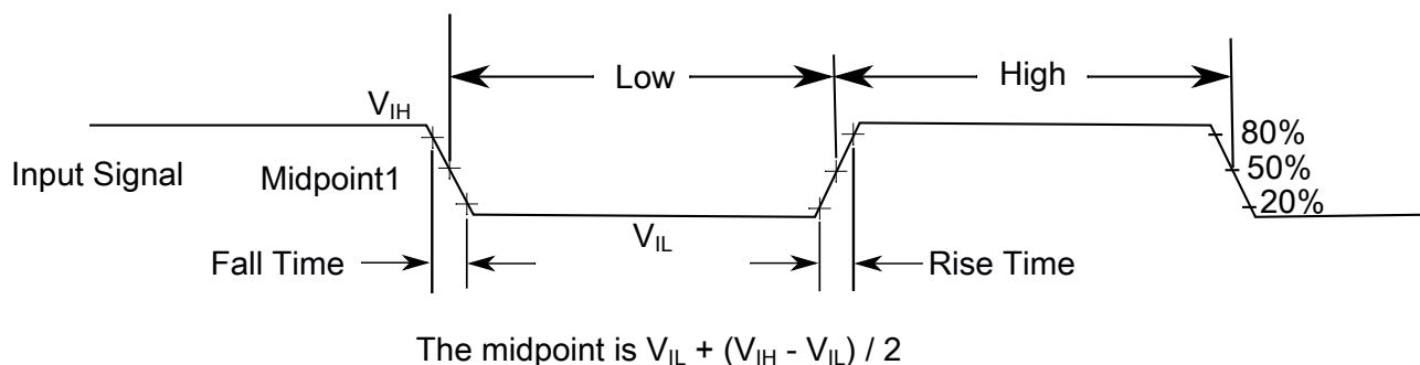
Figure 8. Input signal measurement reference
