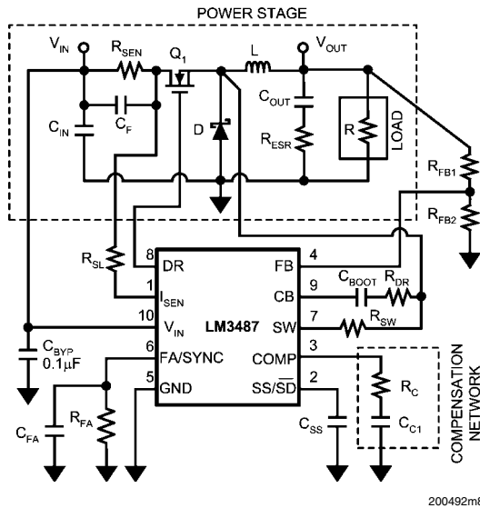
FIGURE 8. LM3487 Buck Converter Reference Schematic
