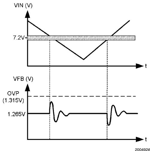
FIGURE 5. The Feedback Voltage Experiences an Oscillation if the Input Voltage Crosses the 7.2V Internal Bias Threshold
