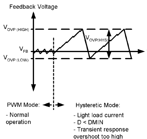
FIGURE 4. The Feedback Voltage is related to the Output Voltage. See different Ripple Components in PWM and Hysteretic Modes
