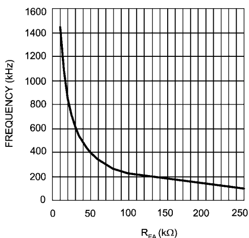
FIGURE 2. Programming the Switching Frequency
