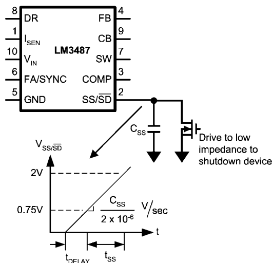
FIGURE 7. Soft Start Thresholds
