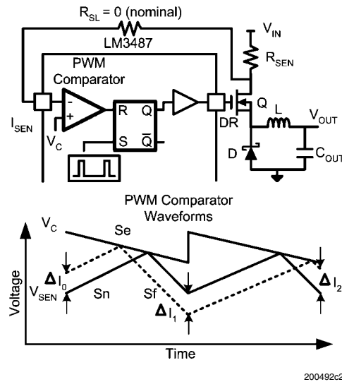
FIGURE 6. The Current Sensing Loop and Corresponding Waveforms
