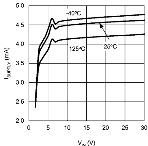
I_{\text{Supply}} vs Temperature & Supply Voltage (Switching)
