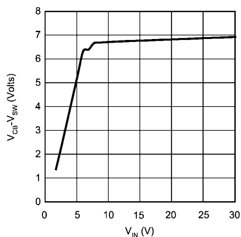
V_{\text{CB}} - V_{\text{SW}} vs Supply Voltage
