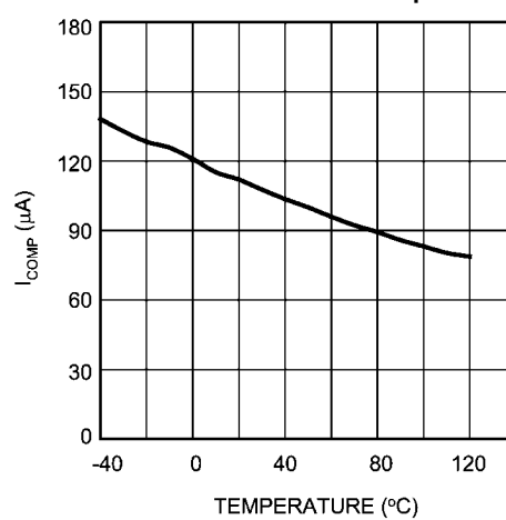
COMP Pin Source Current vs Temperature
