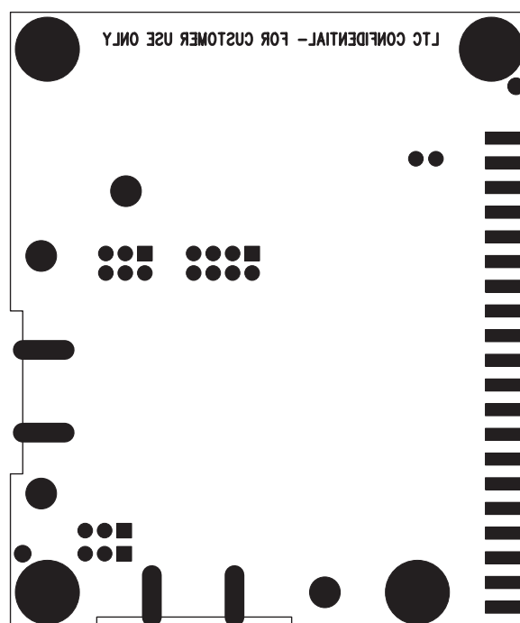
Silkscreen Bottom
