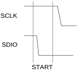
Figure 23: Valid START Condition
