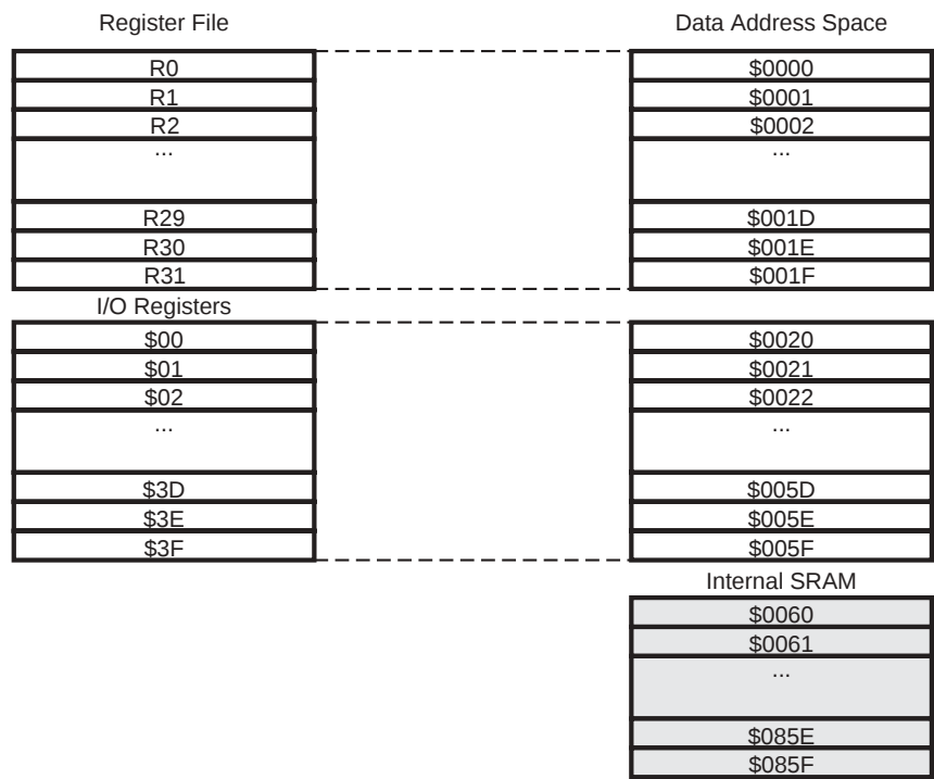
Figure 9. SRAM Organization
