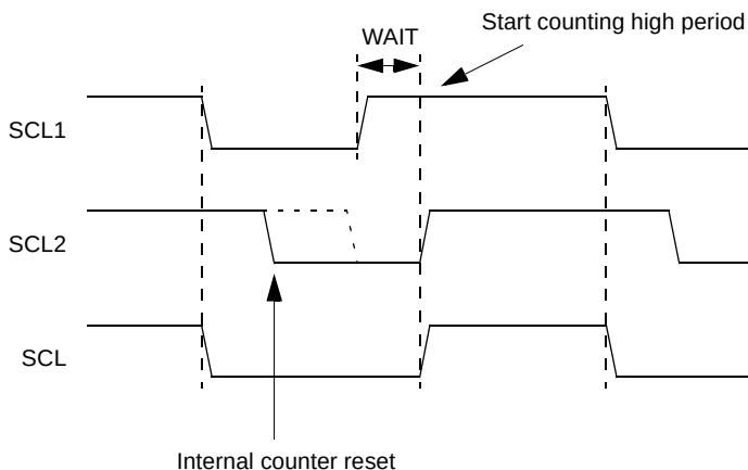
Figure 17-3. Clock Synchronization
