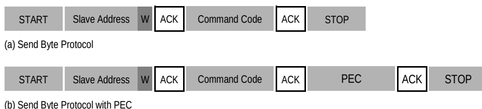
Figure 17-14. Send Byte
