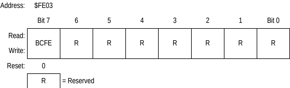
Figure 23-7. SIM Break Flag Control Register (SBFCR)
