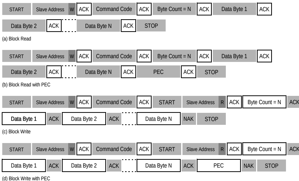
Figure 17-19. Block Read/Write
