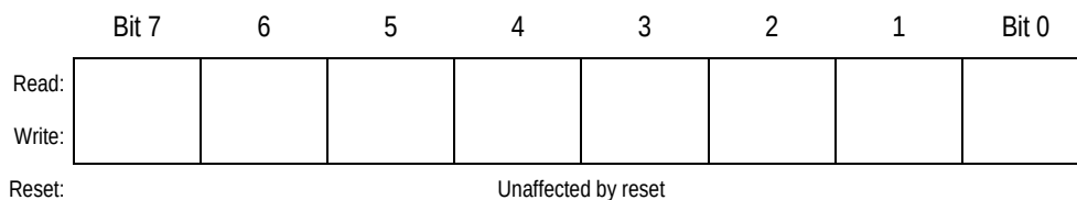
Figure 6-2. Accumulator (A)
