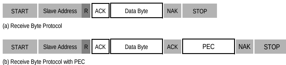
Figure 17-15. Receive Byte
