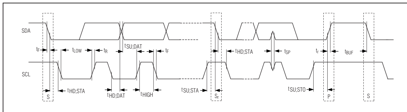
Figure 1. I 2 C Slow-/Fast-Mode Timing Diagram
