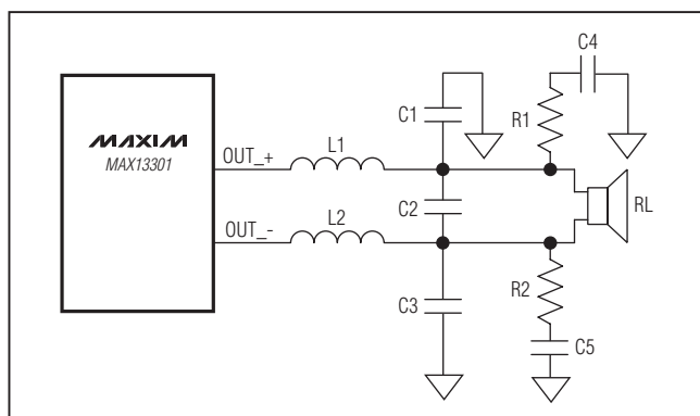
Figure 8. Output Filter
