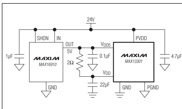
Figure 9. Using a Linear Regulator to Produce 5V from a 24V Power Supply
