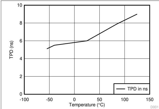
Figure 6-1. TPD vs Temperature at 3.3 V
