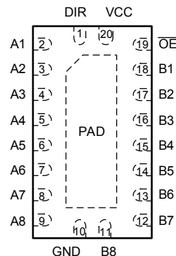
Figure 5-2. SN74AHC245 RKS Package, VQFN 20-Pin (Top View)
