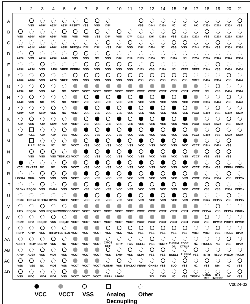
Figure 22. Pin/Ball Map - Top View
