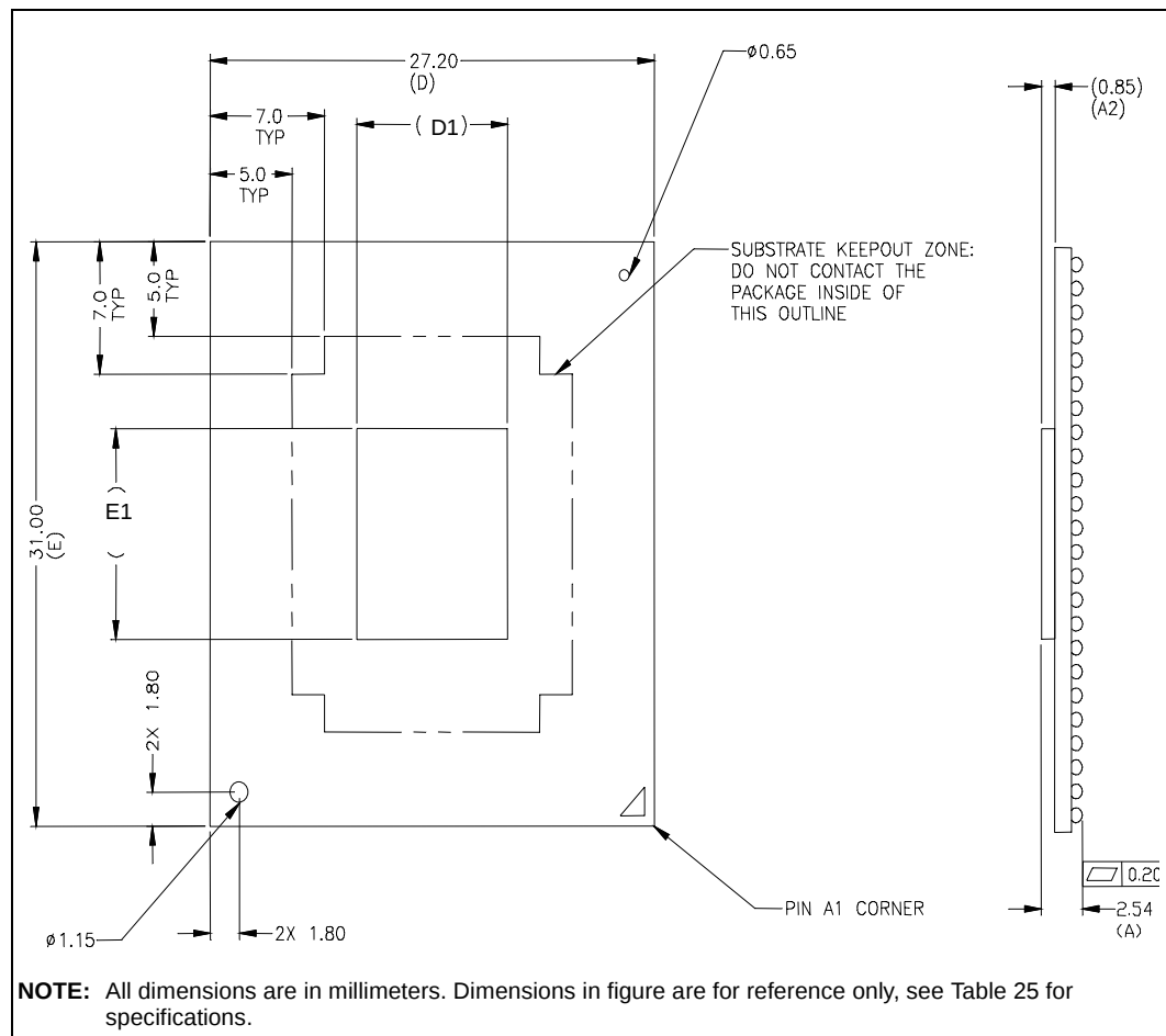
Figure 20. Surface-mount BGA2 Package - Top and Side View
