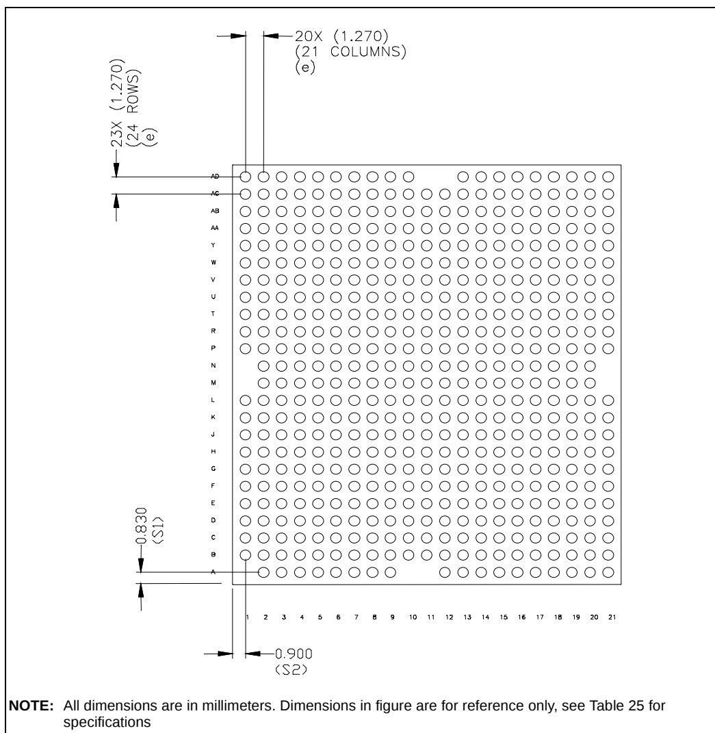
Figure 21. Surface-mount BGA2 Package - Bottom View
