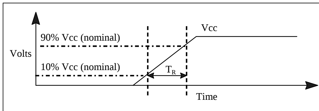
Figure 4. V_{CC} Ramp Rate Requirement
