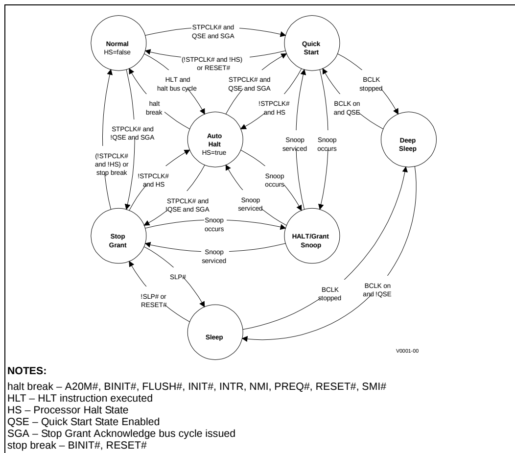
Figure 3. Clock Control States
