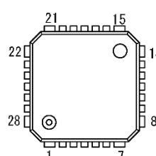
HQFN0808-28 Pin Configuration
