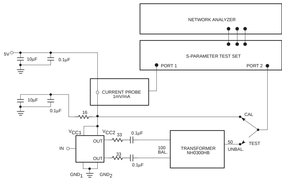
Test Circuit 3
