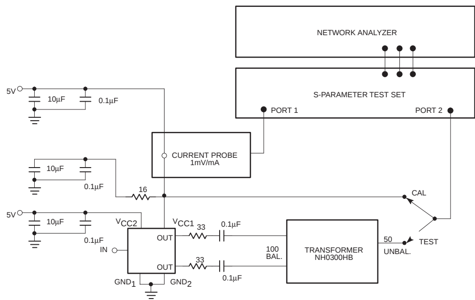
Test Circuit 4
