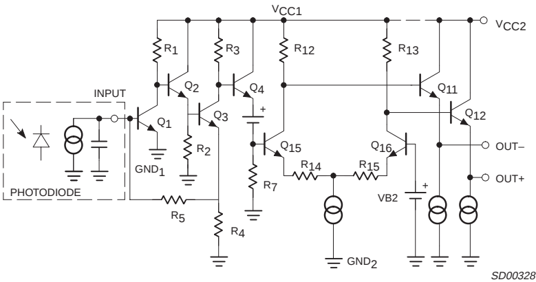
Fig 12. Transimpedance amplifier.
