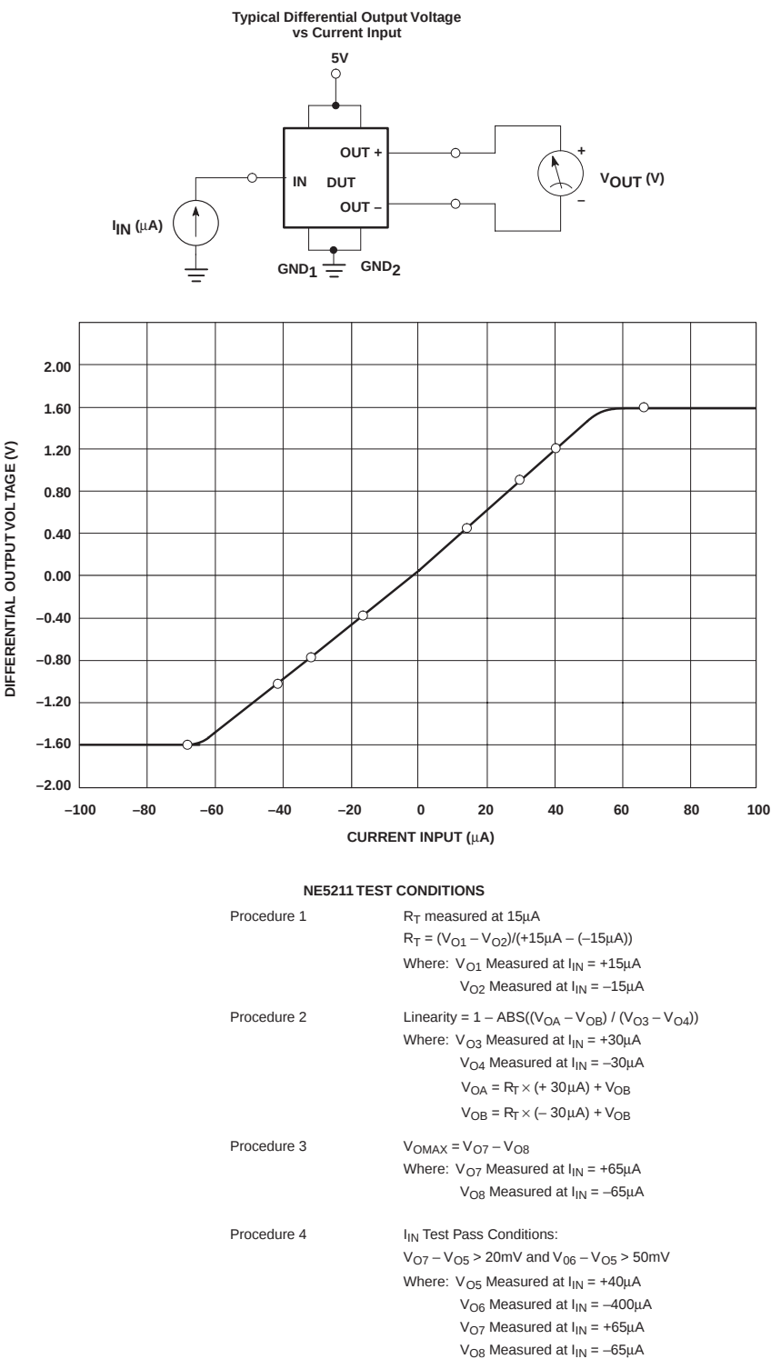
Test Circuit 8
