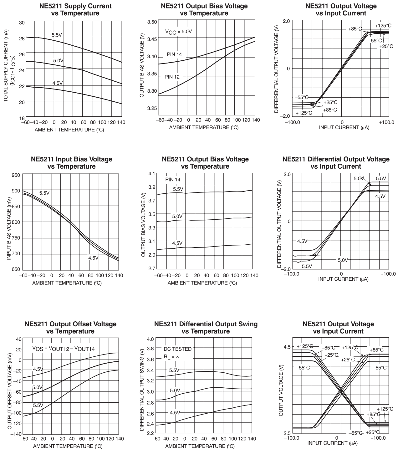
Fig 7. Typical performance characteristics.
