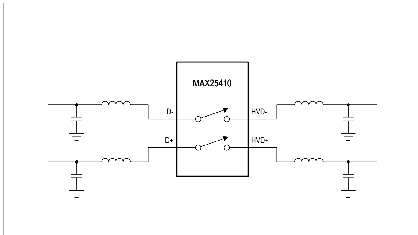
Figure 2. Tuning of Data Lines
