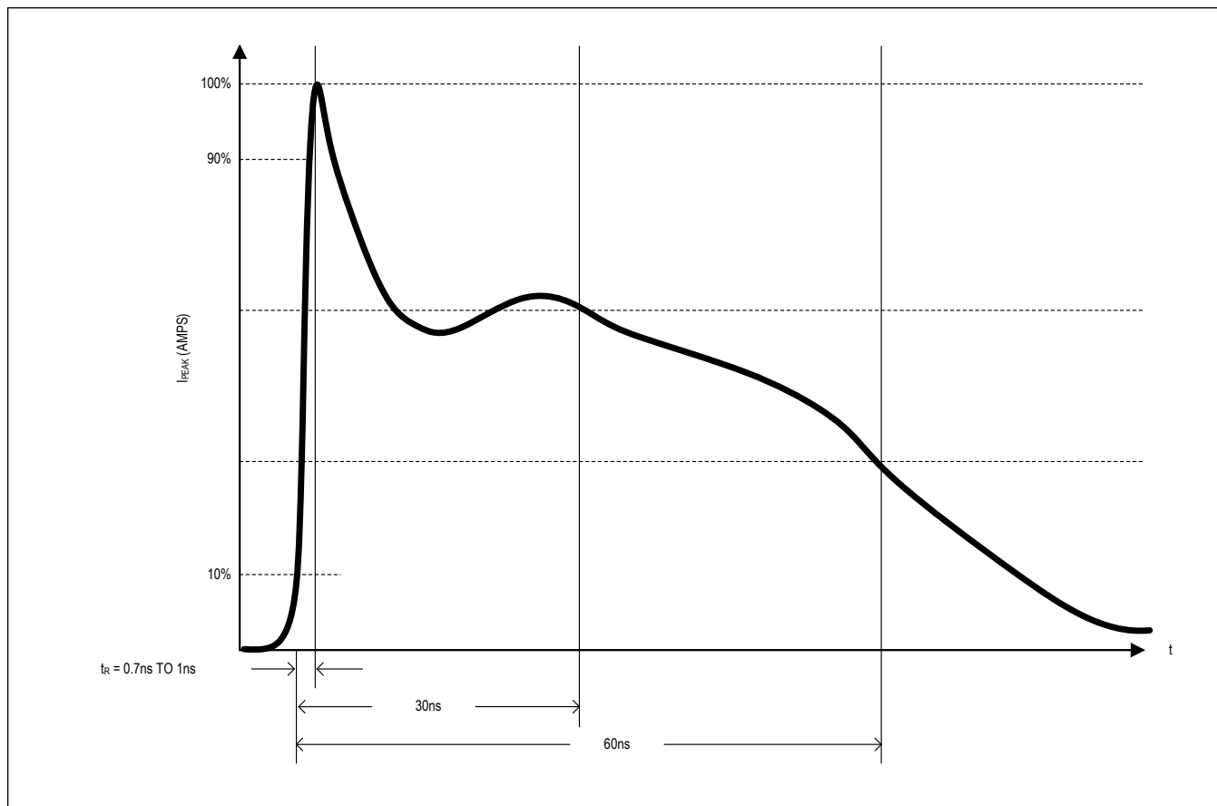
Figure 6. IEC 61000-4-2 ESD Generator Current Waveform
