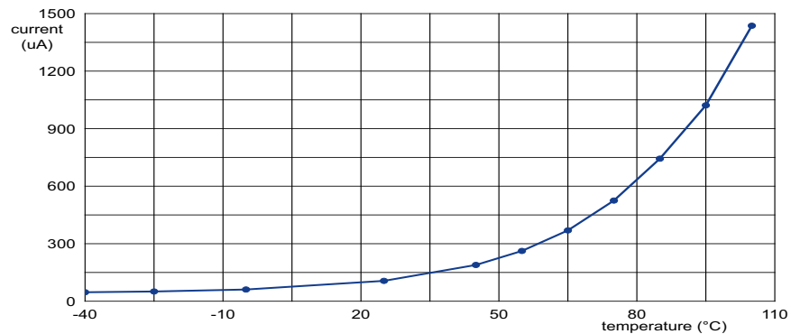
Fig 9. Deep-sleep mode: Typical supply current I_{DD} versus temperature for different supply voltages VBAT_DCDC
