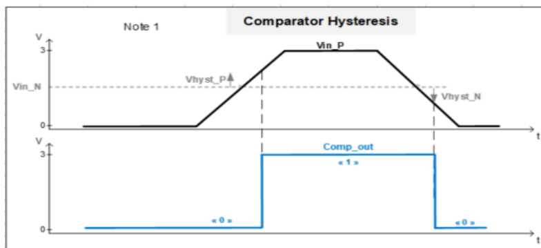
Fig 25. Comparator Hysteresis
