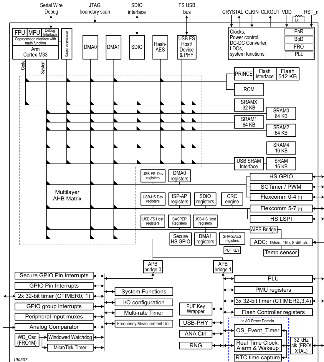
Fig 4. LPC55S2x/LPC552x Block Diagram
