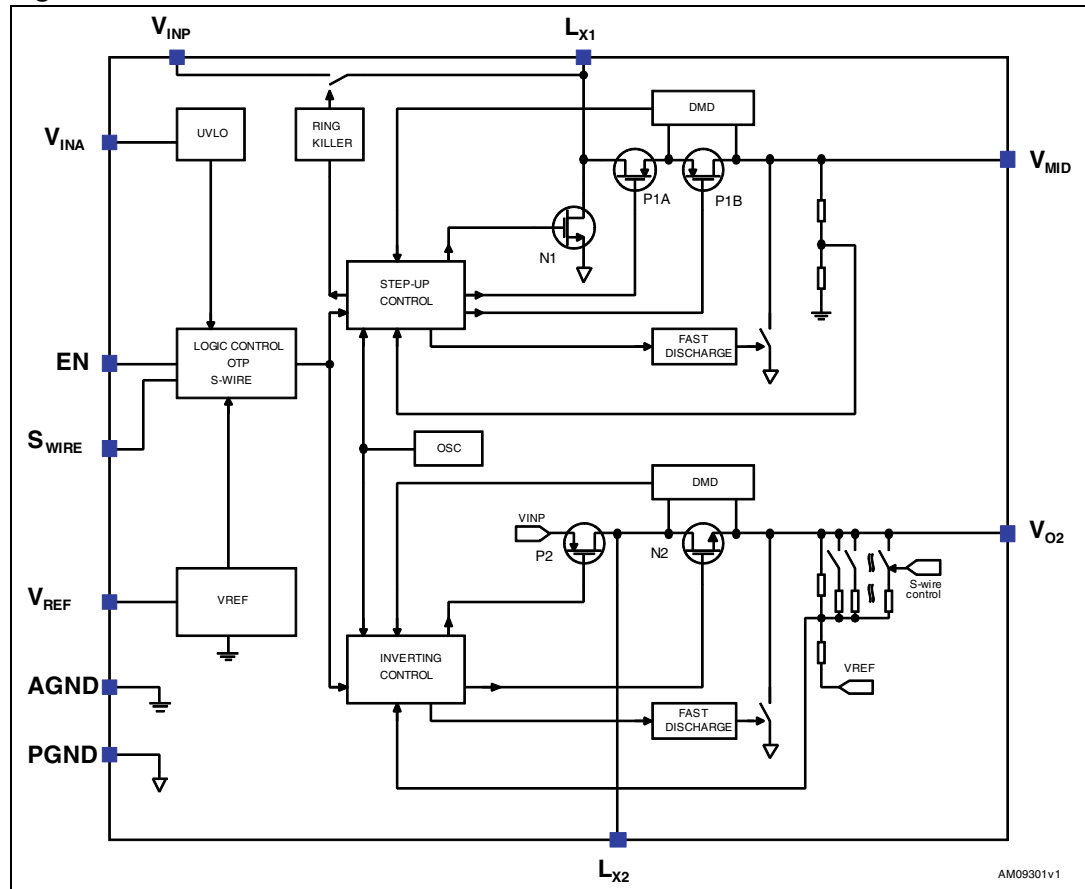
Figure 2. Block schematic
