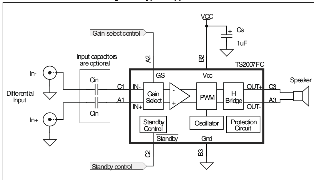
Figure 2. Typical application
