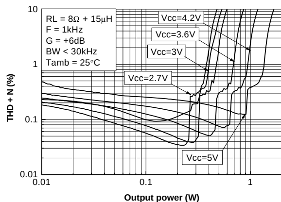
Figure 19. THD+N vs. output power @ 8 \Omega and 1 kHz
