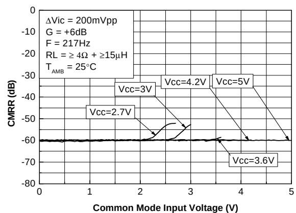
Figure 34. CMRR vs. common mode input voltage @ +6 dB gain
