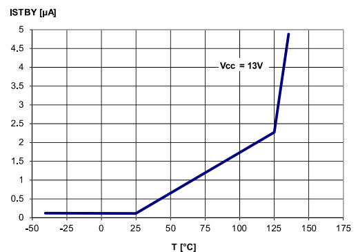
Figure 9: Standby current
