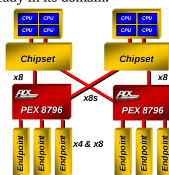
Figure 9. Host Fail-Over
