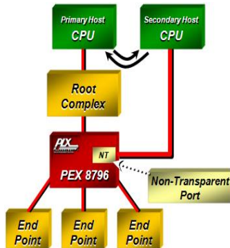
Figure 3: Non-Transparent Port
