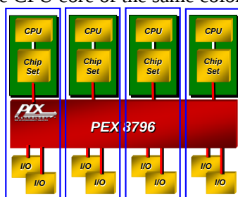
Figure 7. Multi-Host System
