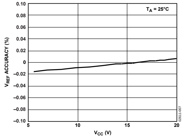
Figure 7. V_{REF} Accuracy vs. V_{CC}
