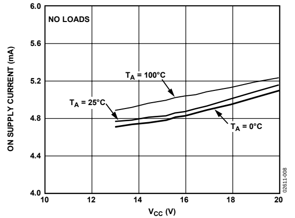
Figure 8. On Supply Current vs. V_{CC}
