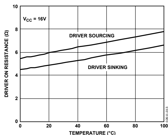
Figure 13. Driver On Resistance vs. Temperature
