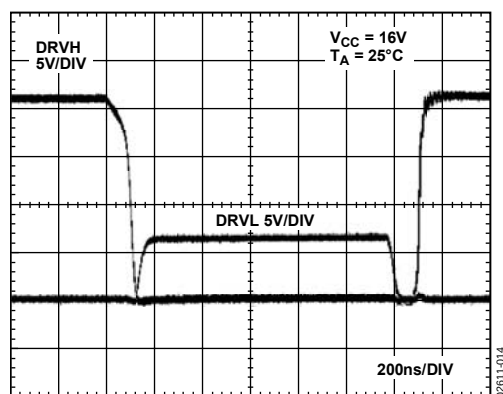
Figure 14. Driver Waveforms
