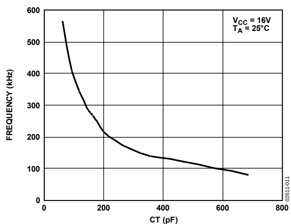
Figure 11. Oscillator Frequency vs. CT
