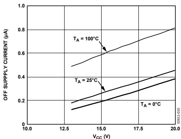
Figure 10. Off Supply Current vs. V_{CC}
