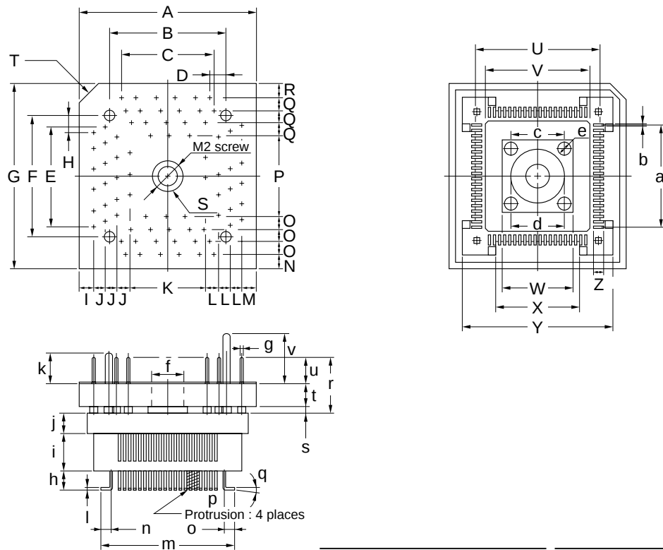
Figure A-3. TGK-080SDW Drawing (For Reference Only)
