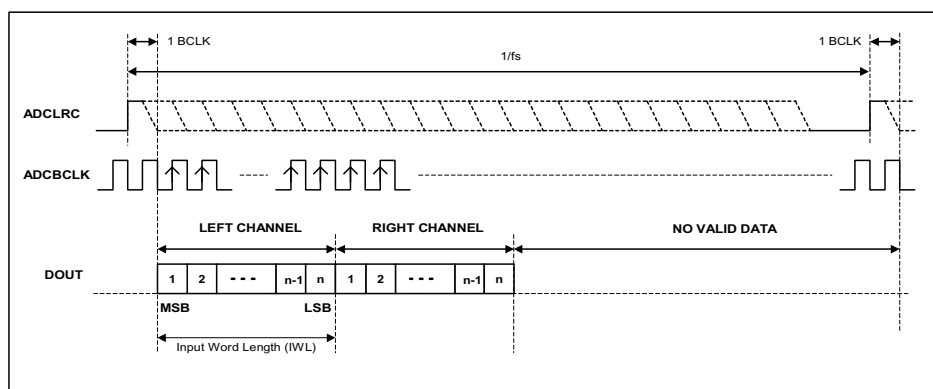
Figure 17 DSP Mode A Timing Diagram – ADC Data Output
