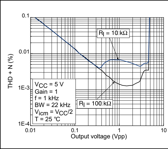
Figure 20. THD+N vs. output voltage
