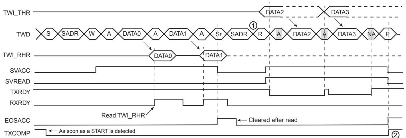
Figure 24-29. Repeated Start + Reversal from Write to Read Mode
