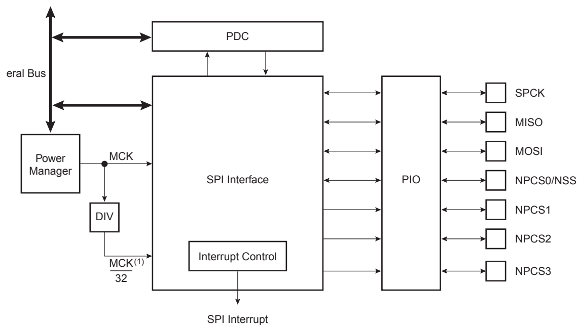
Figure 23-1. Block Diagram
