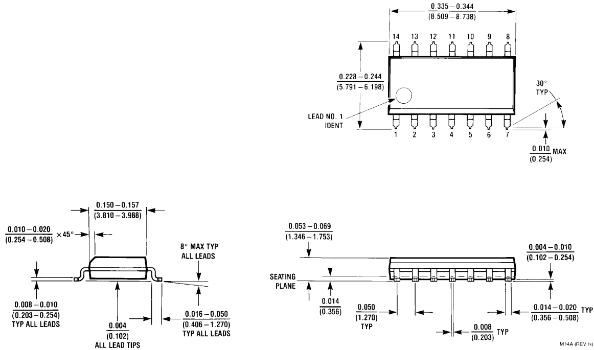
Order Number DS14C88M or DS14C88TM NS Package Number M14A
