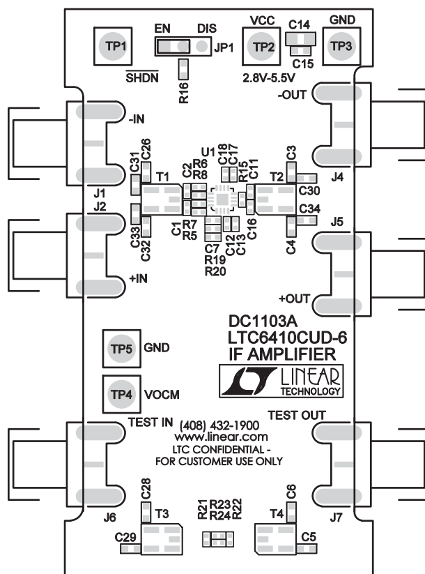
Demoboard DC1103A Top Silkscreen
