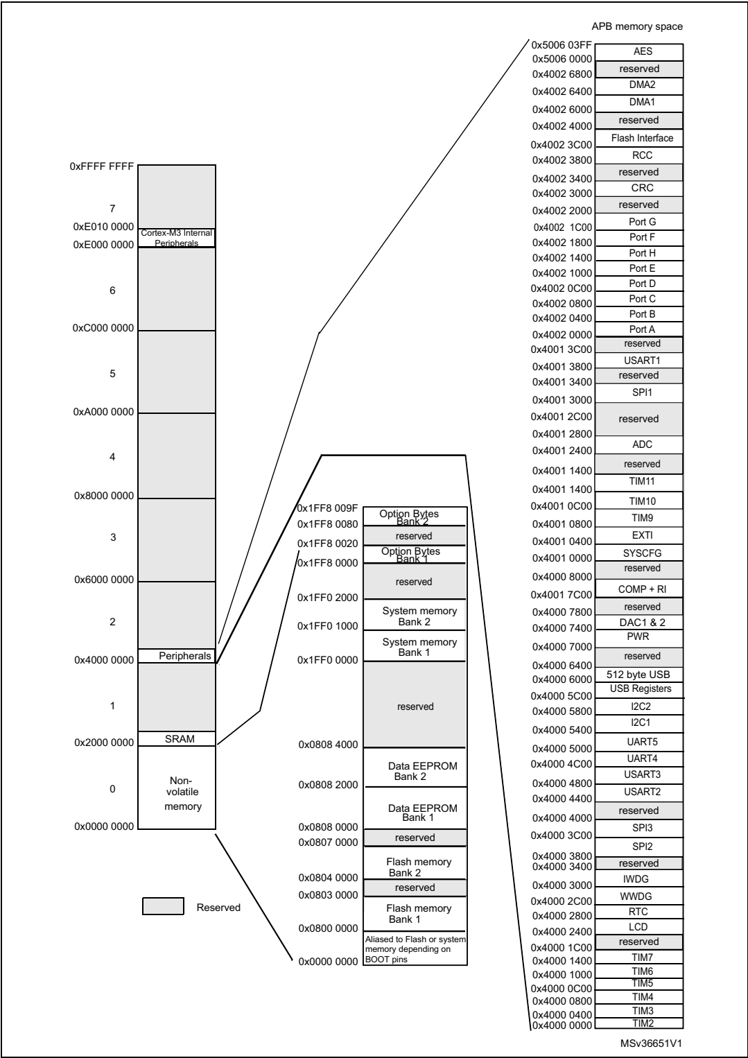
Figure 5. Memory map
