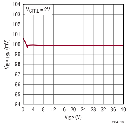
V_{ISP-ISN} vs V_{ISP}
