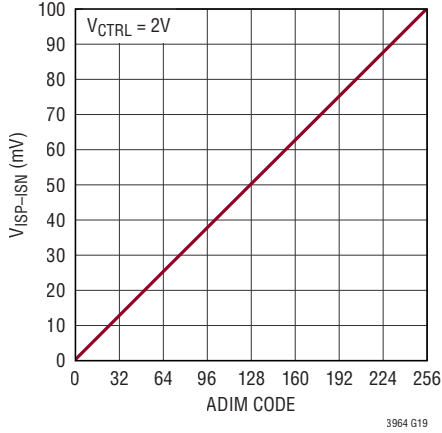
V_{ISP-ISN} vs ADIM
