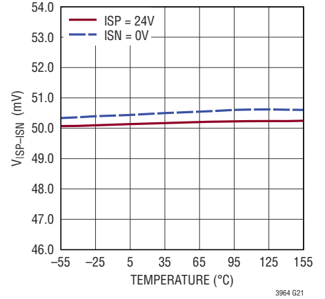
V_{ISP-ISN} 1/2 Scale ( V_{CTRL} = 0.7V ) vs Temperature
