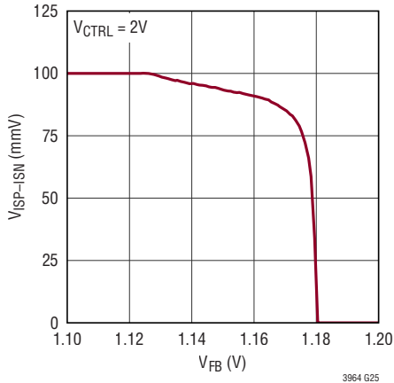
V_{ISP-ISN} vs V_{FB}
