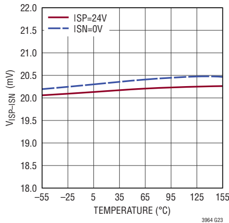
V_{ISP-ISN} 1/5 Scale ( V_{CTRL} = 0.4V ) vs Temperature
