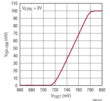
V_{ISP-ISN} vs V_{TSET} at 90^\circ\text{C}
