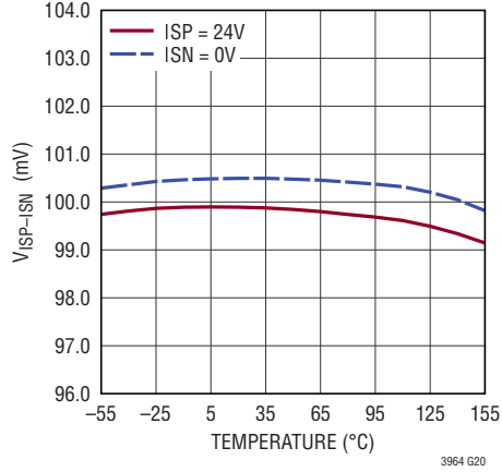
V_{ISP-ISN} Full Scale vs Temperature
