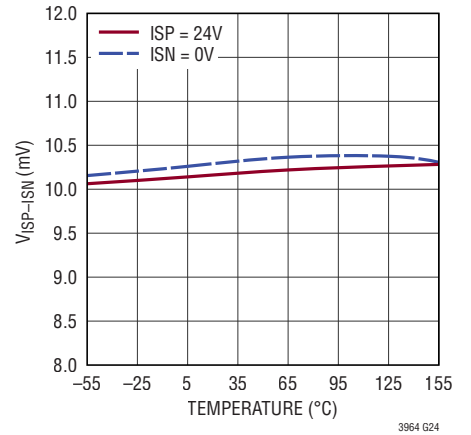
V_{ISP-ISN} 1/10 Scale ( V_{CTRL} = 0.3V ) vs Temperature
