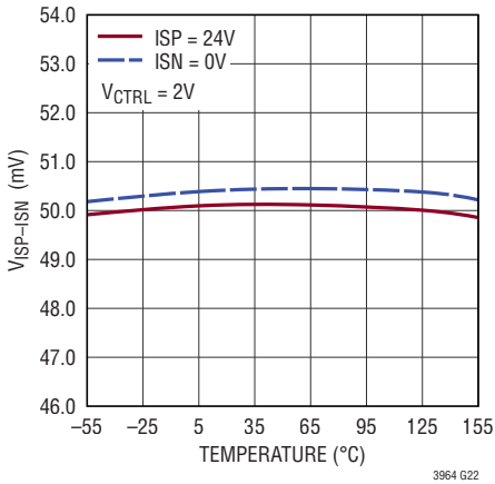
V_{ISP-ISN} 1/2 Scale (ADIM = 0x7f) vs Temperature
