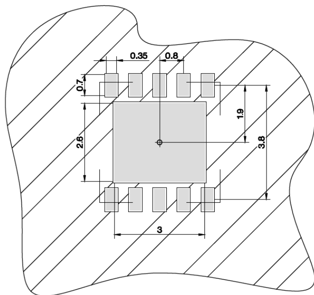
PG-WSO-10-1: Boardpads & Apertures
