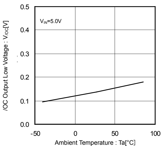
Figure 11. /OC Output Low Voltage vs Ambient Temperature
