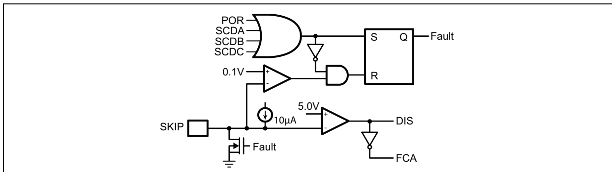
FIGURE 3-5: TIMER CIRCUIT
