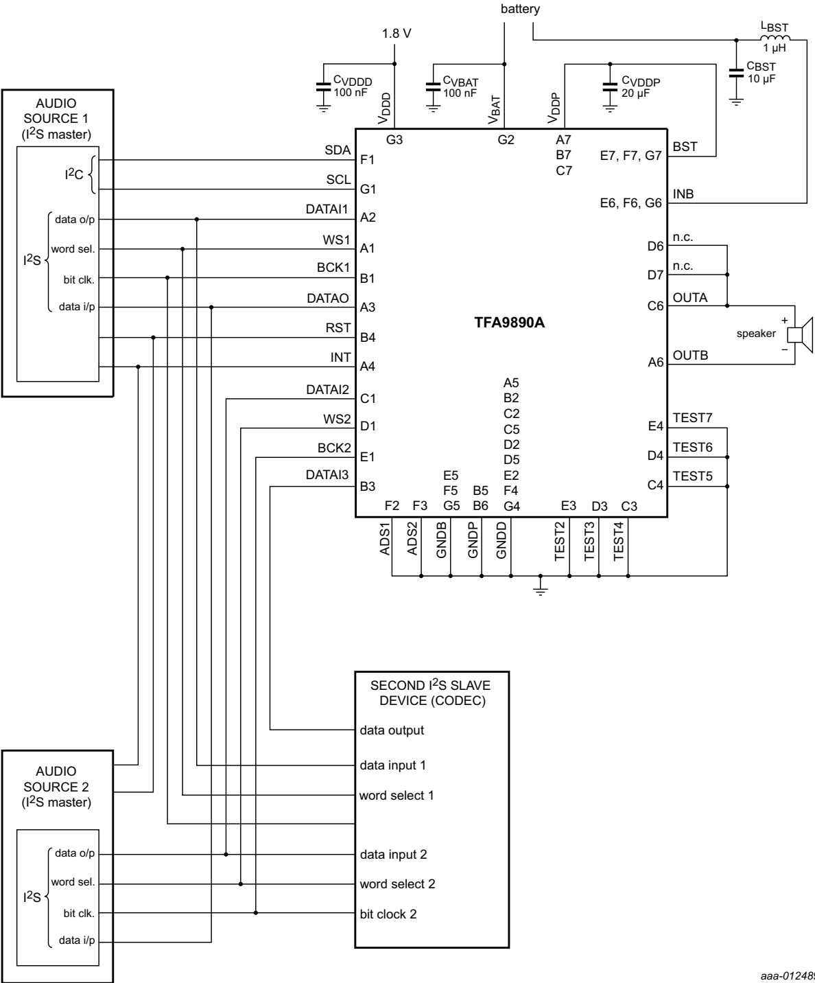
Fig 9. Typical mono application with two audio sources and a second I2S slave device
