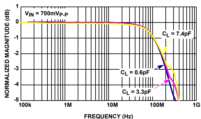
FIGURE 8. LARGE SIGNAL GAIN FLATNESS, GAIN = 2
