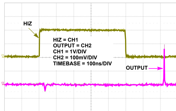
FIGURE 26. HIZ SWITCHING GLITCH, V_{IN} = 0 , GAIN = 2
