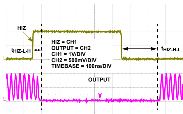
FIGURE 27. HIZ TIMING, GAIN = 1
