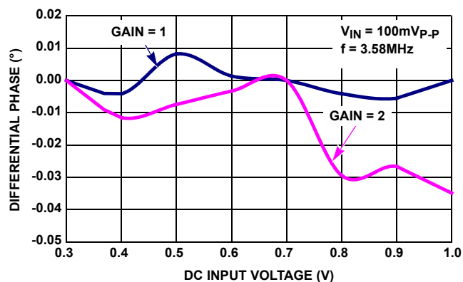
FIGURE 20. DIFFERENTIAL PHASE; f_O = 3.58MHz , R_L = 150\Omega
