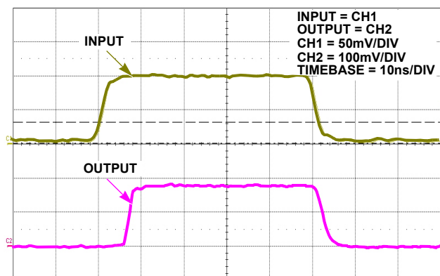
FIGURE 22. SMALL SIGNAL TRANSIENT RESPONSE; GAIN = 2
