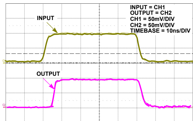
FIGURE 21. SMALL SIGNAL TRANSIENT RESPONSE; GAIN = 1
