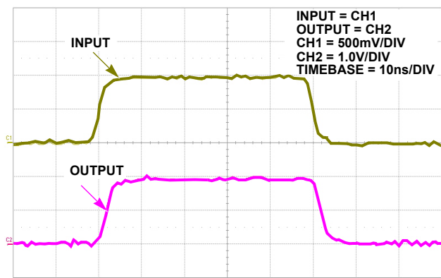
FIGURE 24. LARGE SIGNAL TRANSIENT RESPONSE; GAIN = 2
