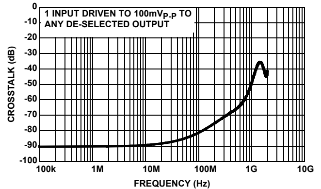
FIGURE 16. OFF ISOLATION
