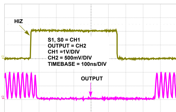
FIGURE 28. HIZ TIMING, GAIN = 2
