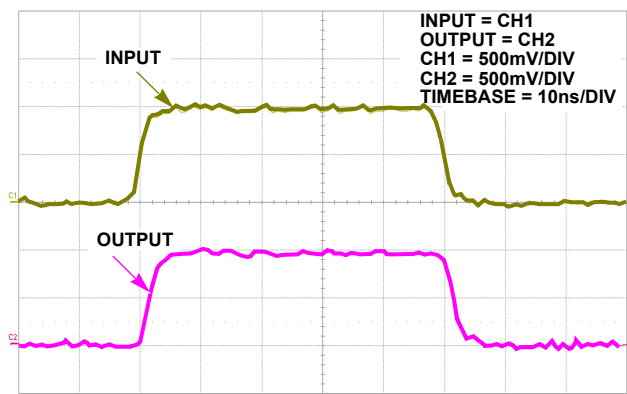
FIGURE 23. LARGE SIGNAL TRANSIENT RESPONSE; GAIN = 1
