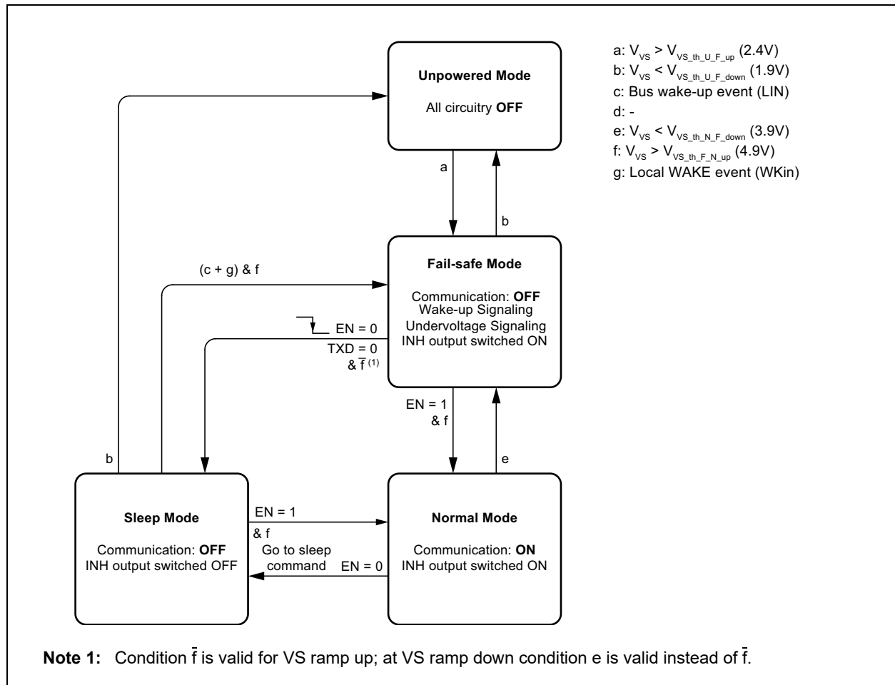
FIGURE 1-1: ATA663211 OPERATING MODES
