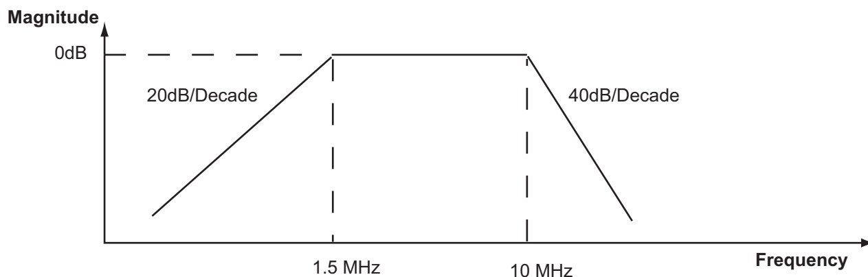
Figure 5: Weighing function for RMS Phase Jitter Calculation
