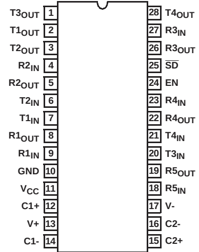
HIN213E (SOIC, SSOP) TOP VIEW
