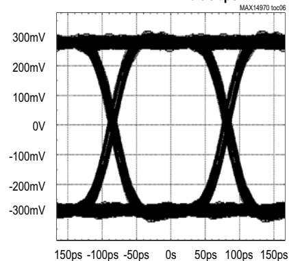
VRX-DFF-PP = 1000mVp-p, PA = GND, DATA RATE = 6.0Gbps
