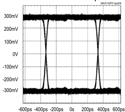
VRX-DFF-PP = 1000mVp-p, PA = GND, DATA RATE = 1.5Gbps
