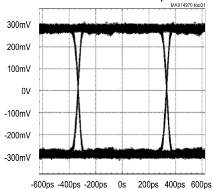
VRX-DFF-PP = 240mVp-p, PA = GND, DATA RATE = 1.5Gbps
