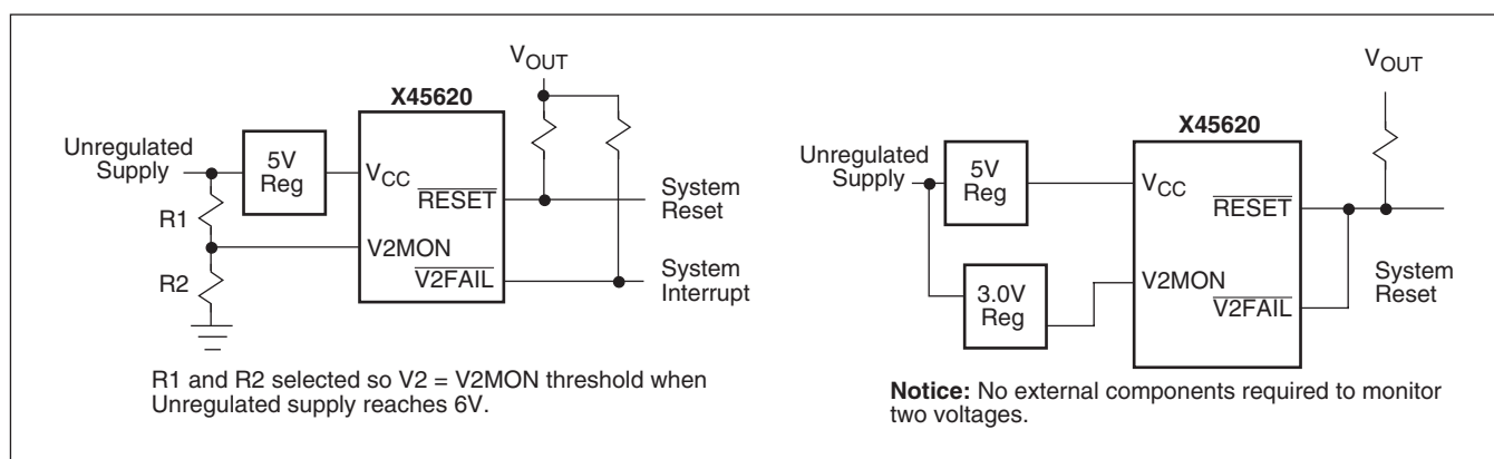
Figure 1. Two Uses of Dual Voltage Monitoring
