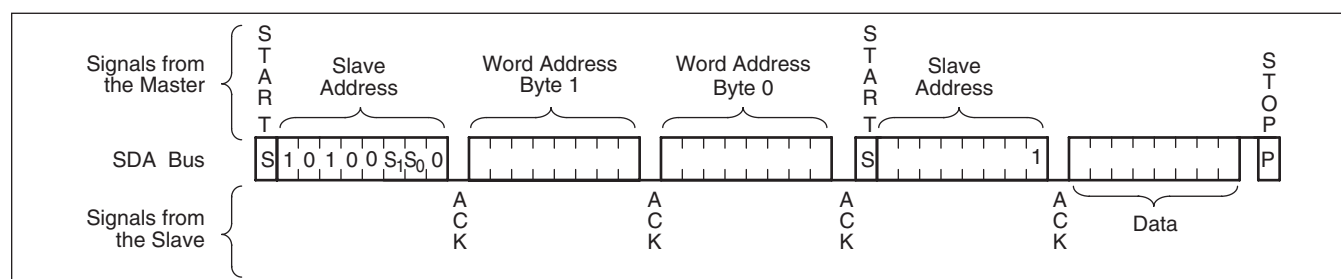
Figure 15. Random Read Sequence
