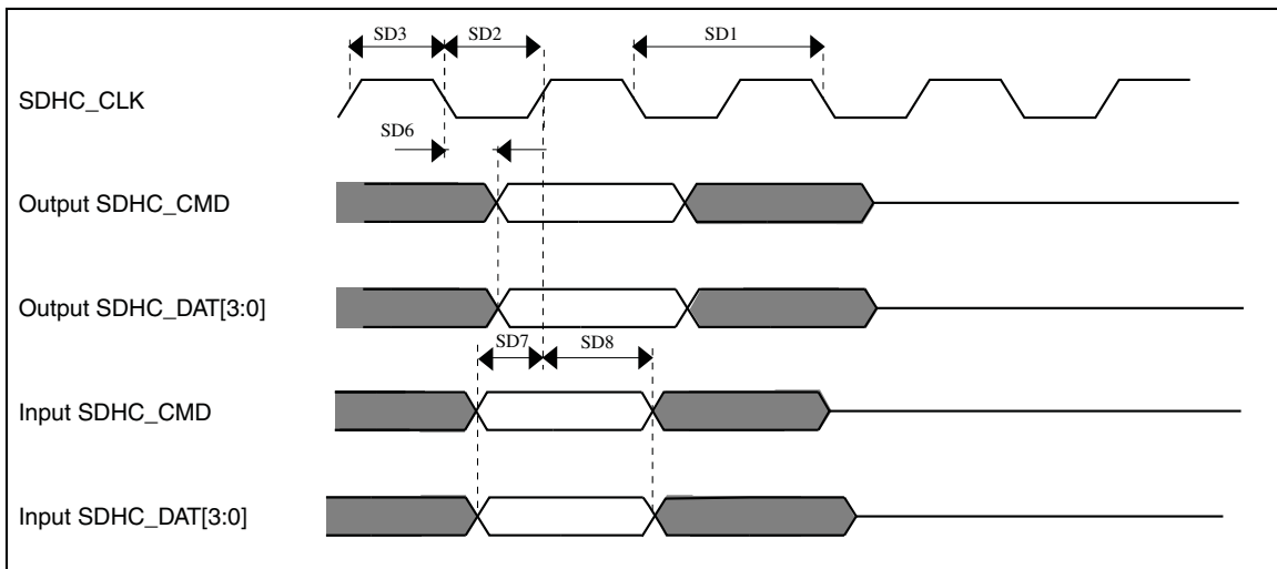
Figure 53. SDHC timing
