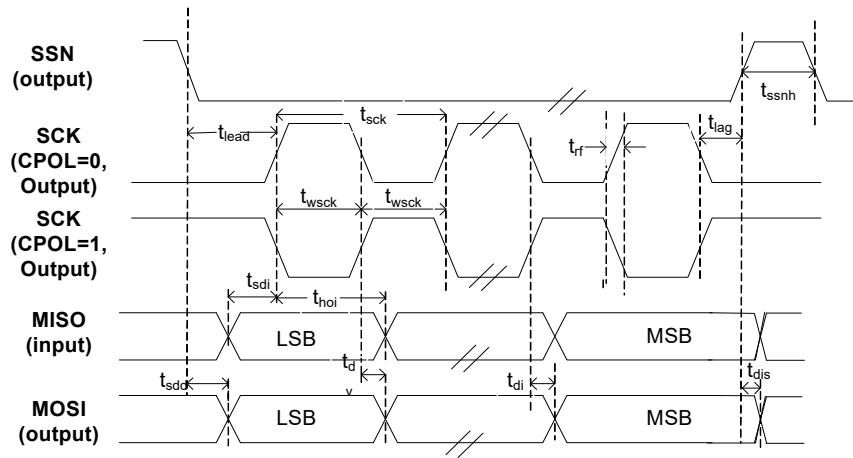
Figure 14. SPI Timing
