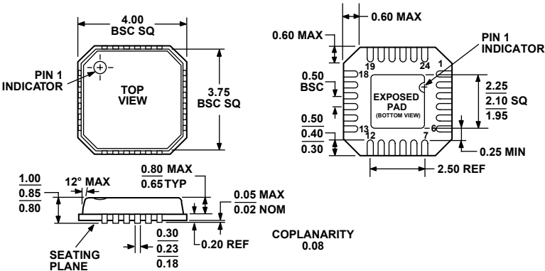
COMPLIANT TO JEDEC STANDARDS MO-220-VGGD-2 Figure 20. 24-Lead Lead Frame Chip Scale Package [LFCSP_VQ] 4 mm × 4 mm Body, Very Thin Quad (CP-24-1) Dimensions shown in millimeters
