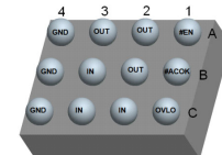
WLCSP-12 CASE 567WP
