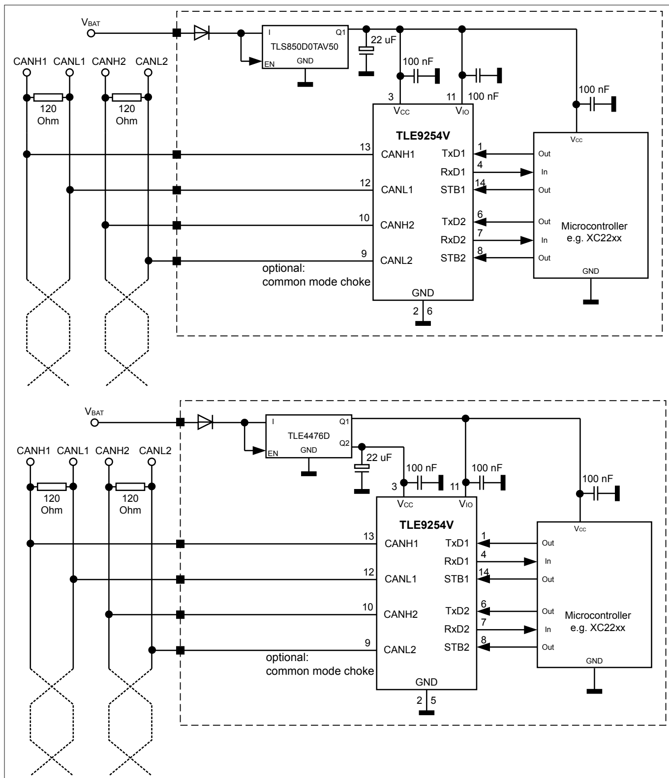
Figure 17 Application circuit
