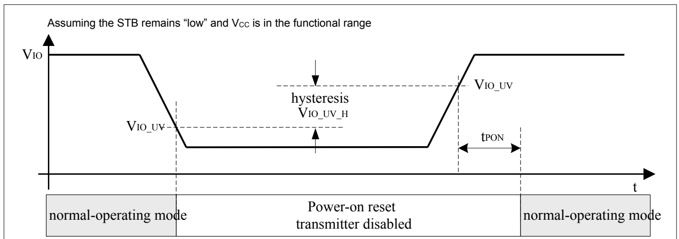
Figure 13 V_{IO} undervoltage
