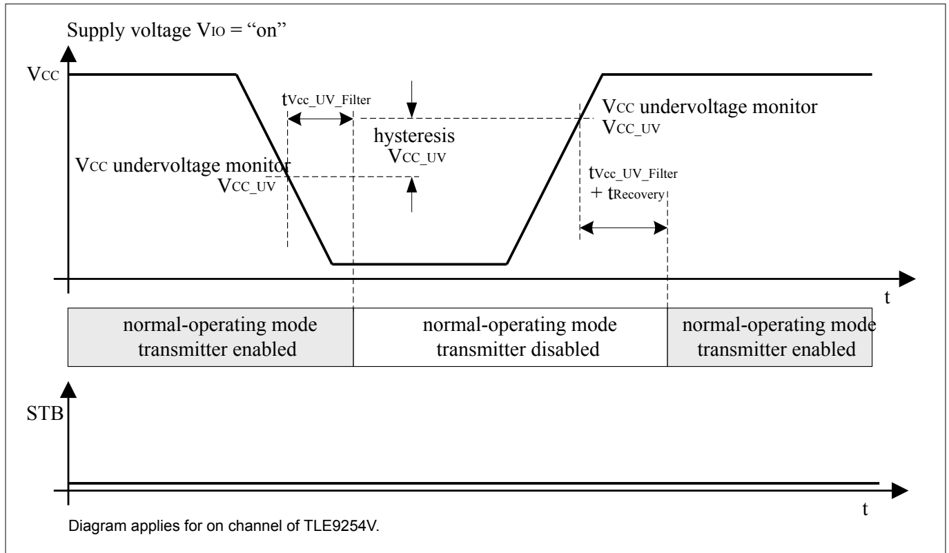
Figure 12 V_{CC} undervoltage
