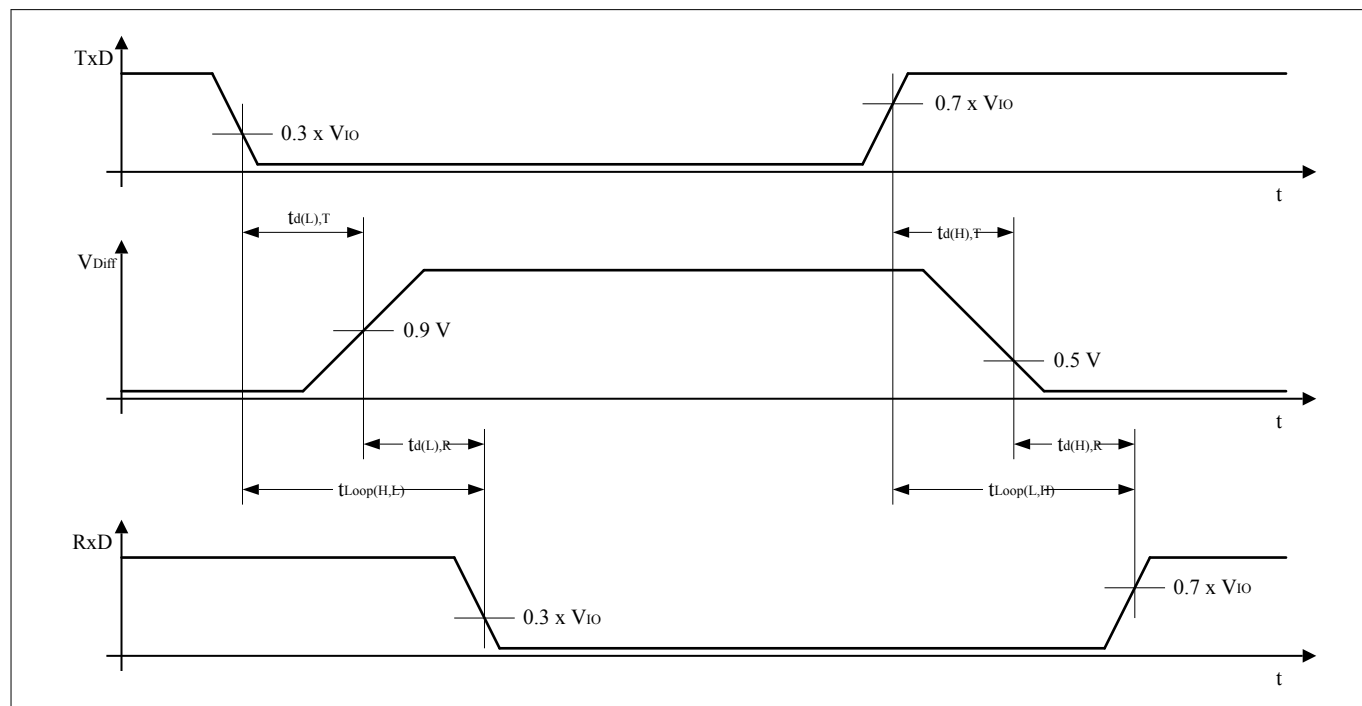
Figure 15 Timing diagram for dynamic characteristics
