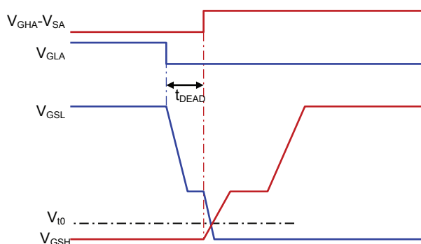
Figure 7: Minimum Dead Time
