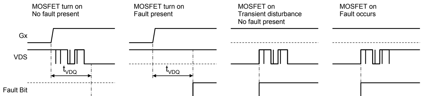
Figure 5a: VDS Fault Monitor – Blank Mode Timing (VDQ = 1)
