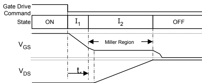
Figure 6c: On-to-Off Transition (Gate Drive)
