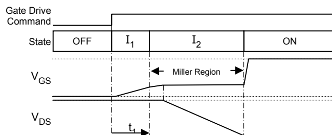
Figure 6a: Off-to-On Transition (Gate Drive)
