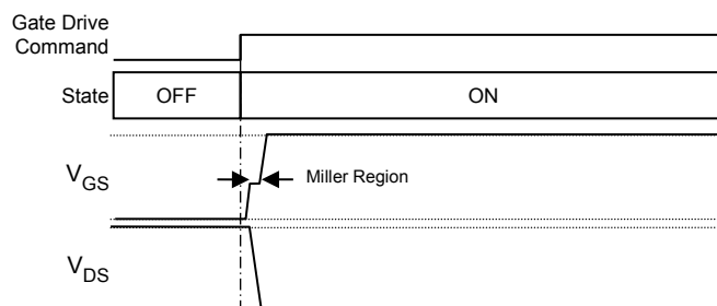
Figure 6b: Off-to-On Transition (Switched)
