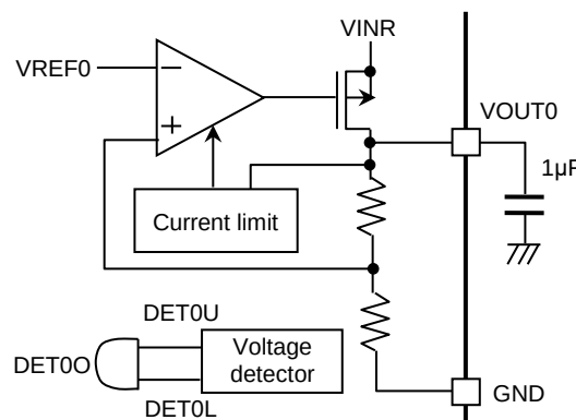
Figure 4-8 LDO0 block diagram
