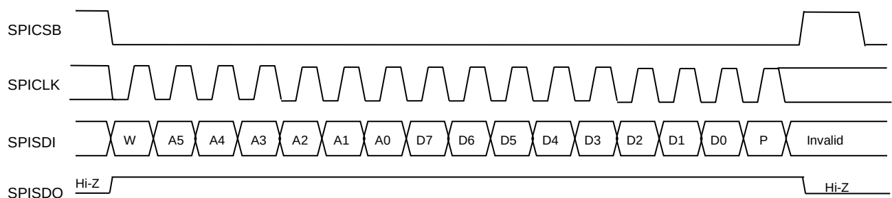
Figure 4-2 SPI format (Write)
