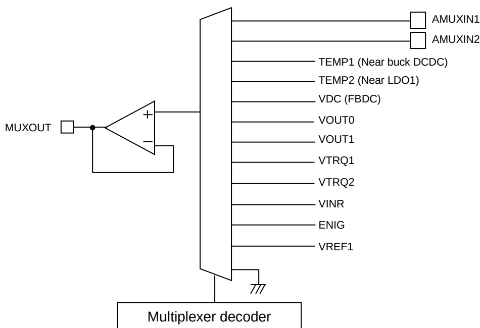
Figure 4-54 Diagram of analog monitoring
