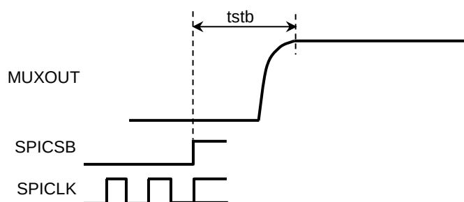
Figure 4-56 Output timing
