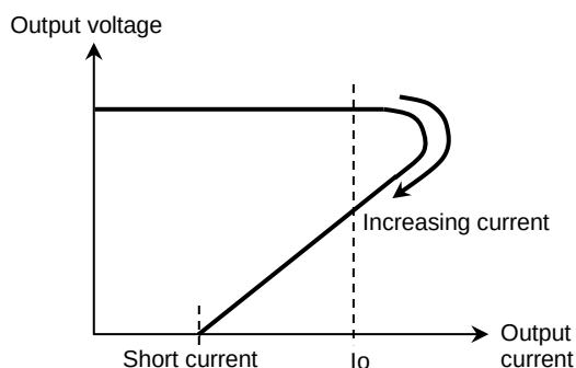
Figure 4-10 Fold-back characteristic
