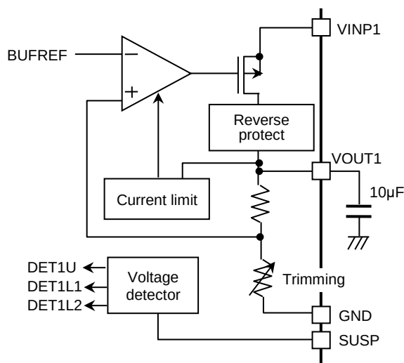
Figure 4-9 LDO1 block diagram
