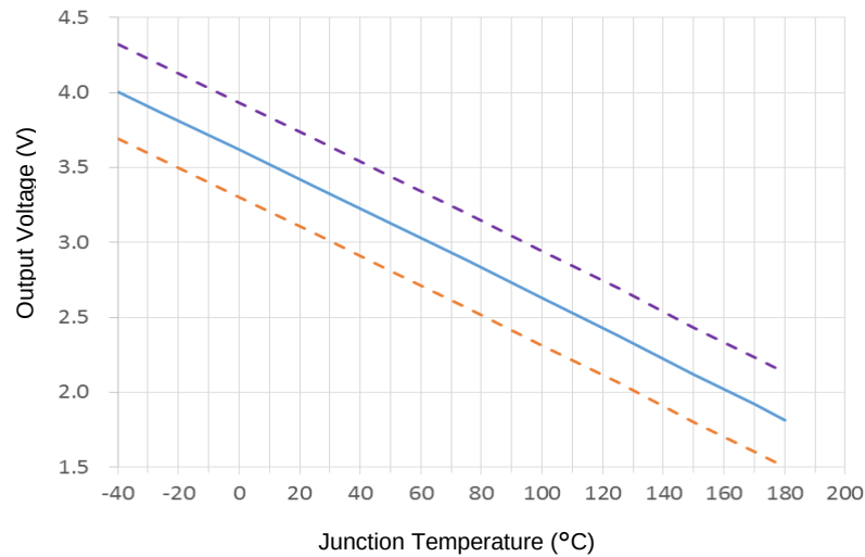
Figure 4-57 Output of temperature sensor
