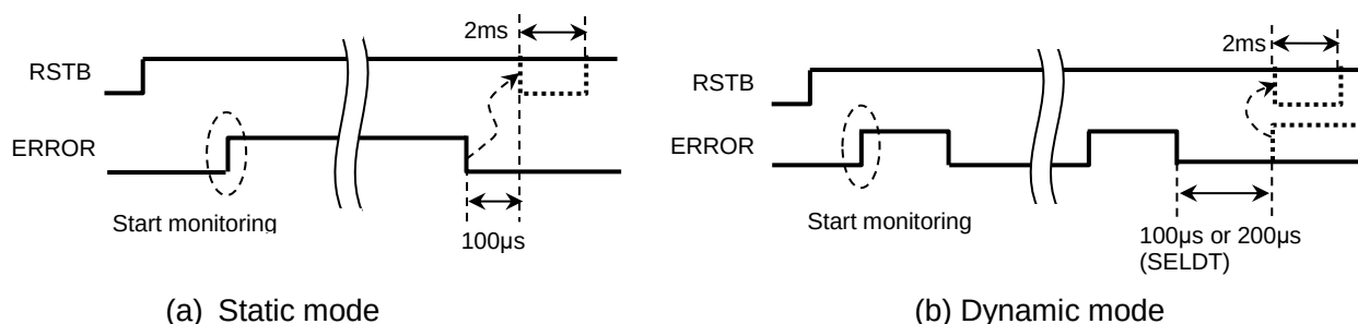
Figure 4-43 ERROR behavior
