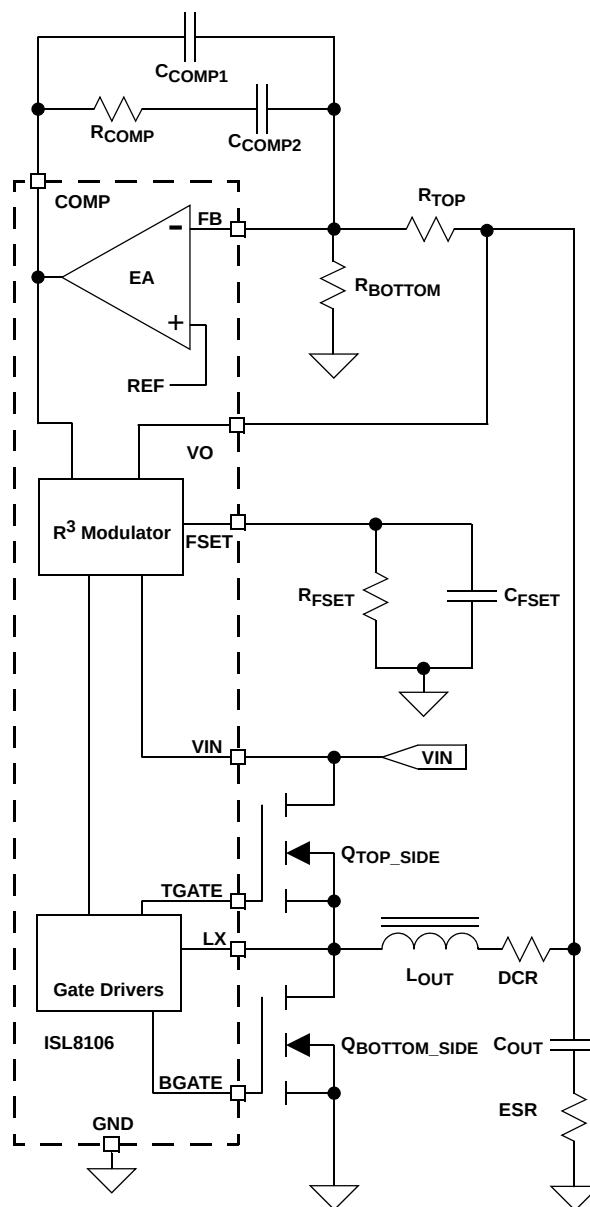
FIGURE 7. COMPENSATION REFERENCE CIRCUIT
