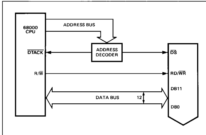
FIGURE 6: 68000 16-Bit Microprocessor to DAC-8012 Interface
