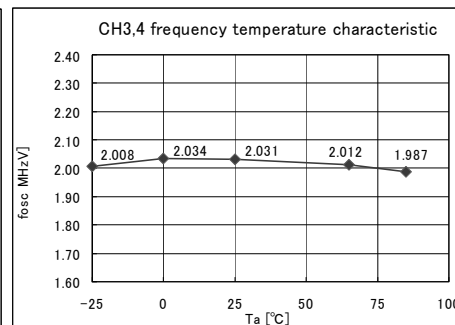
Fig.4 Frequency CH3,4—Temp
