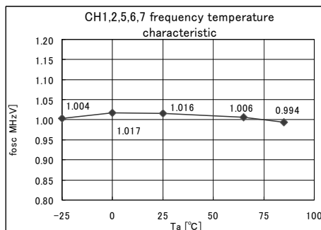
Fig.3 Frequency CH1,2,5~7—Temp
