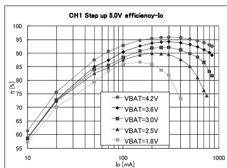
Fig.6 CH1 5.0V voltage boost efficiency—I o
