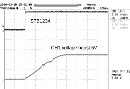
Fig.15 CH1 start-up waveform (VBAT=3.6V)
