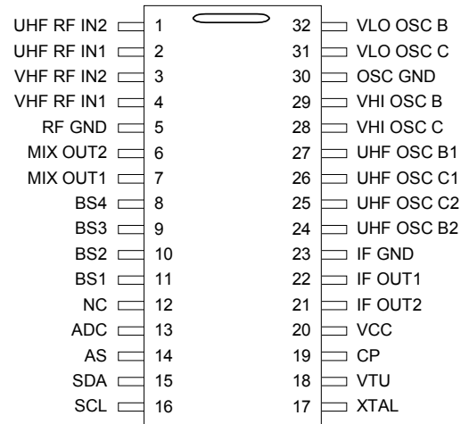
DAE package (TOP VIEW) 32PIN TSSOP (DAE)
