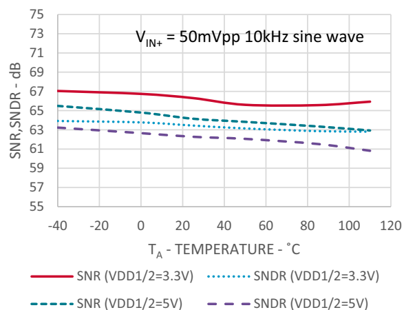
Figure 15: SNR, SNDR vs. Temperature
