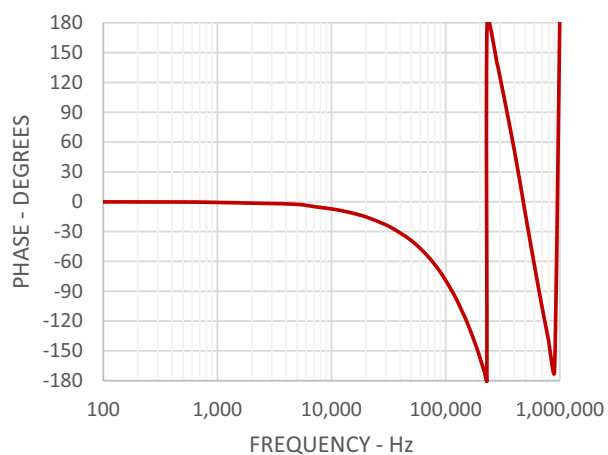
Figure 18: Phase Frequency Response
