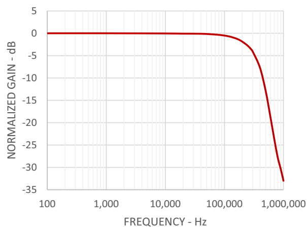
Figure 17: Gain Frequency Response
