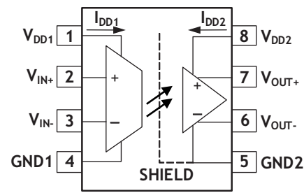
Figure 1: Pin Configuration
