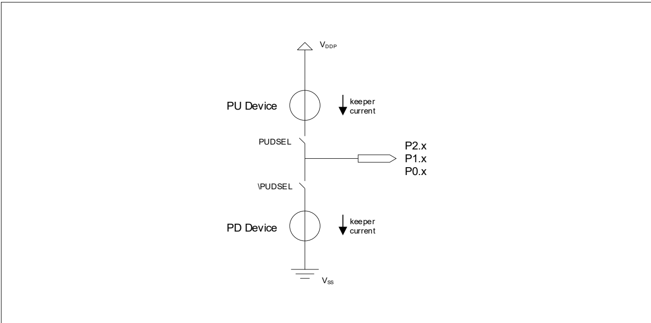
Figure 43 Pull-Up/Down Device
